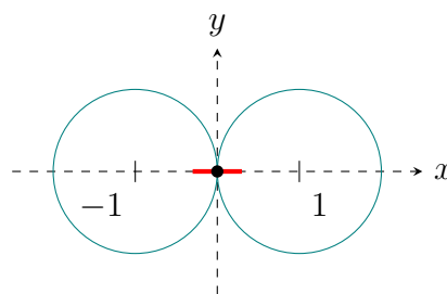
(b) X_2 = C((-1, 0), 1) \cup C((1, 0), 1)
